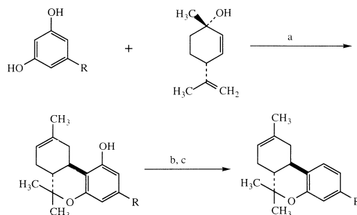
Scheme 2. (a) HOTs/C 6 H 6 , 80°C; (b) NaH/THF, 0°C then (C 2 H 5 O) 2 P(O)Cl; (c) Li/NH 3 , THF, -78°C.
