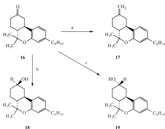
Scheme 3. (a) (C 6 H 5 ) 3 PCH 3 + Br − , n -BuLi/THF, 65°C; (b) LiAlH 4 /THF, 25°C; (c) KBH( sec -Bu) 3 /THF, −78 to 25°C then H 2 O 2 /NaOH.
