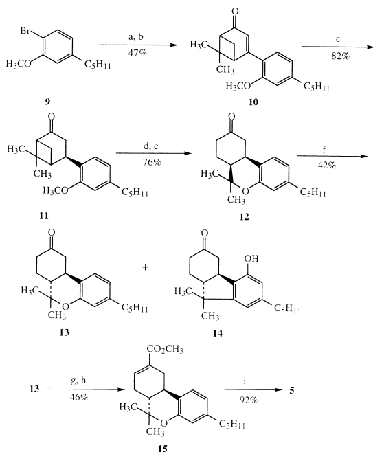
Scheme 1. (a) BuLi/THF, 0°C then apoverbenone; (b) PDC/CH 2 Cl 2 , 25°C; (c) Li/NH 3 , THF, -78°C; (d) NaSP/DMF, 120°C; (e) SnCl 4 /CH 2 Cl 2 , 25°C; (f) AlCl 3 /CH 2 Cl 2 , 25°C; (g) Tf 2 O, 2,6-di- tert -butyl-4-methyl-pyridine/CH 2 Cl 2 , 40°C; (h) Et 3 N, Pd(OAc) 2 , Ph 3 P, CO, CH 3 OH/DMF, 45°C; (i) LiAlH 4 /Et 2 O, 0–25°C.
